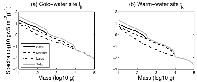
Figure 4. Steady state biomass spectra at two sites. Black solid, dashed, and dash-dot curves represent the small, medium, and large group biomass, respectively, whereas the grey curves represent the total of the three groups. The model is forced at two sites with annual average net primary production (NPP) and temperature ( T ) with a timestep of 15 days. Simulations are for a (a) cold-water site in the East Bering Sea LME (64° N, 165° W) and a (b) warm-water site in the Benguela Current LME site (20° S, 12° E).
