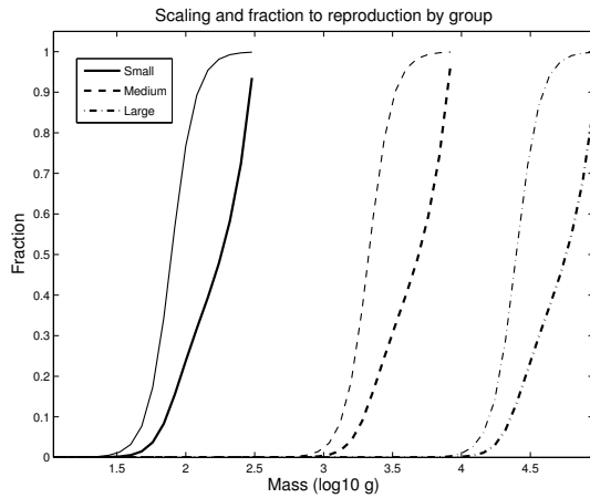
Figure 2. Mass dependence of reproduction by group. The mass scaling function s_k(m) (thin lines, Eq. 23) determines the mass dependence of the allocation of energy to reproduction. \Phi_k(m) (thick lines, Eq. 21) is the fraction of energy allocated to reproduction.
