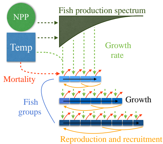
Figure 1. Schematic diagram of the main modules, components, and processes of the ecological module of BOATS. Net primary production (NPP) and temperature ( T ) force the model and are used to calculate the fish production spectrum, by assuming a transfer of energy from phytoplankton to successive sizes of fish that depends on the trophic efficiency and the predator to prey mass ratio. From fish production, we calculate the size-dependent growth rate of biomass in three independent groups that represent small, medium, and large commercial fish. Mortality rates are calculated as a function of size and asymptotic size, and also depend on temperature. Adult fish, the largest sizes in each spectrum, allocate energy to reproduction, of which a fraction is returned to the smallest mass class of the corresponding spectrum, representing recruitment of juveniles.
